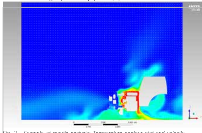
Fig. 3— Example of results analysis: Temperature contour plot and velocity vectors projected on a longitudinal midplane.
