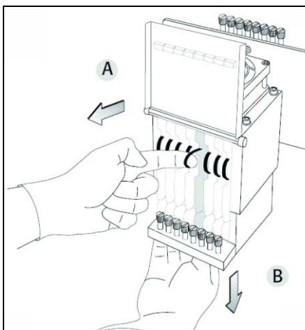
Figure 6-61: Releasing the print-head driver card to remove the head
