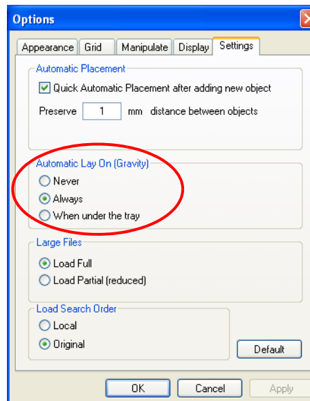
Figure 5-36: Options dialog box, Settings tab
