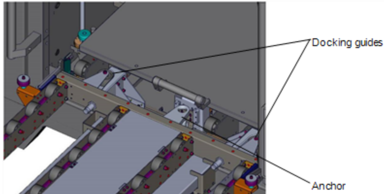
Figure 7-1 Positioning the cart for tray removal
