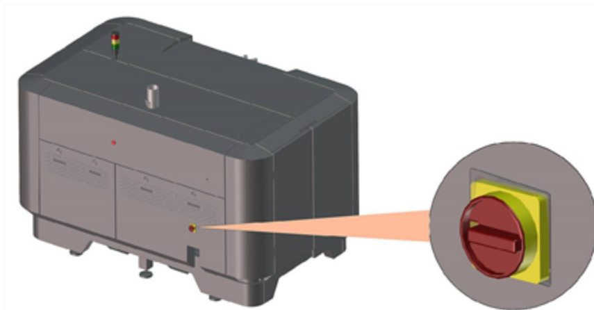
Figure 6-2 Main power switch
