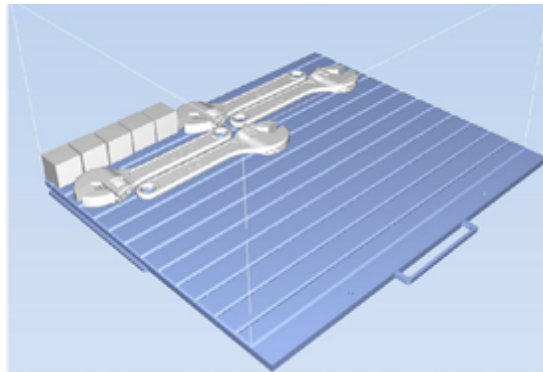
Figure 5-34 Tray arrangement after applying Automatic Placement
