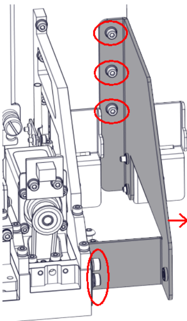
Figure 6-32 Removing the UV bracket
