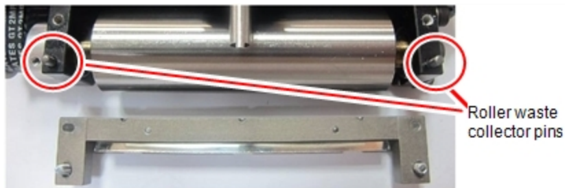
Figure 6-36 Roller waste collector pins
