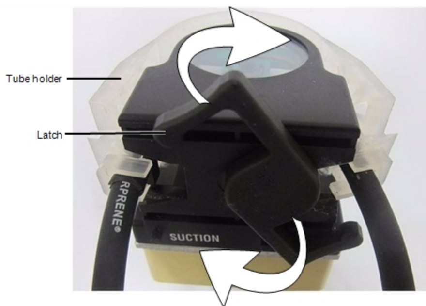
Figure 6-92 Releasing the tube latch
