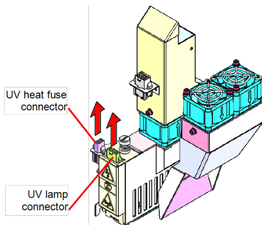
Figure 6-103 Disconnecting the UV lamp
