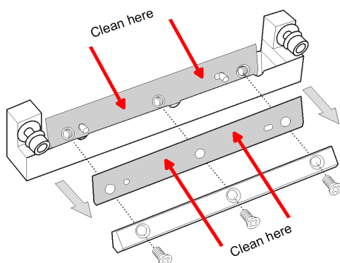
Figure 6-40 Removing the old roller scraper blade
