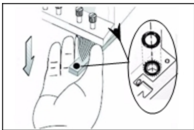
Figure 6-74 O-ring seals on the print head
