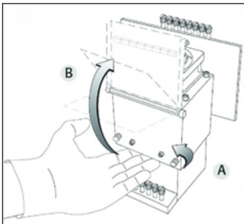
Figure 6-72 Opening the print-head compartment
