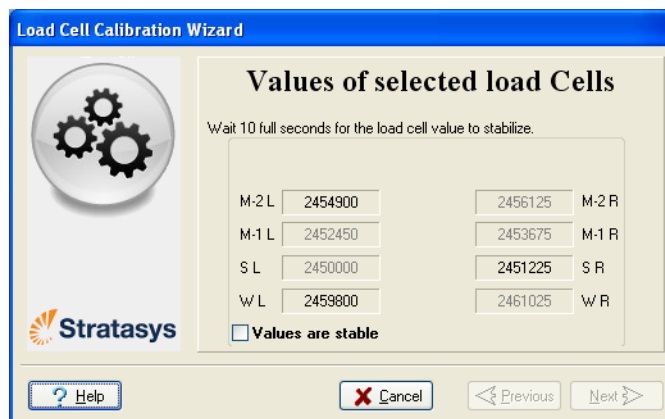
Figure 6-98 Weight stabilization
