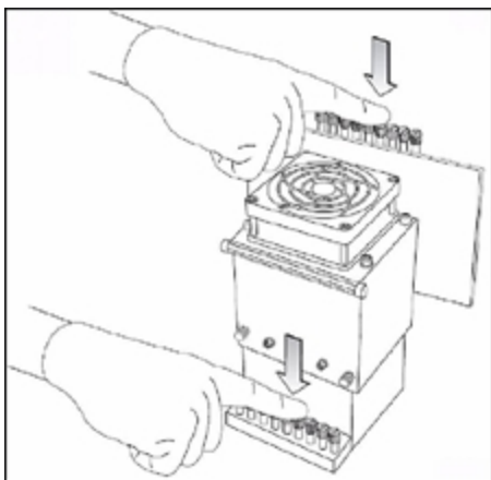
Figure 6-71 Releasing the print head
