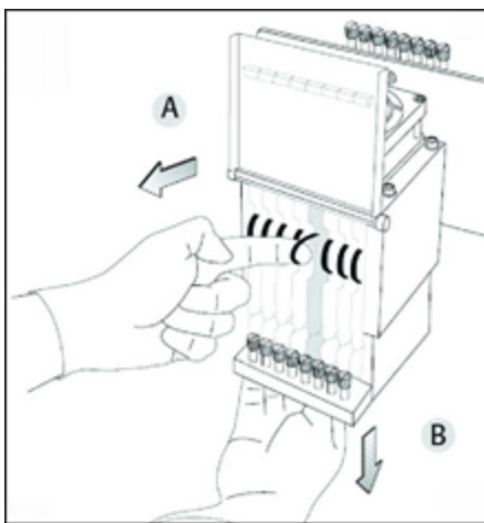
Figure 6-73 Releasing the print-head driver card to remove the head
