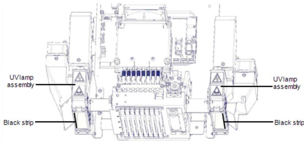
Figure 6-106 Print block and UV lamp assembly, showing correct placement of black strip
