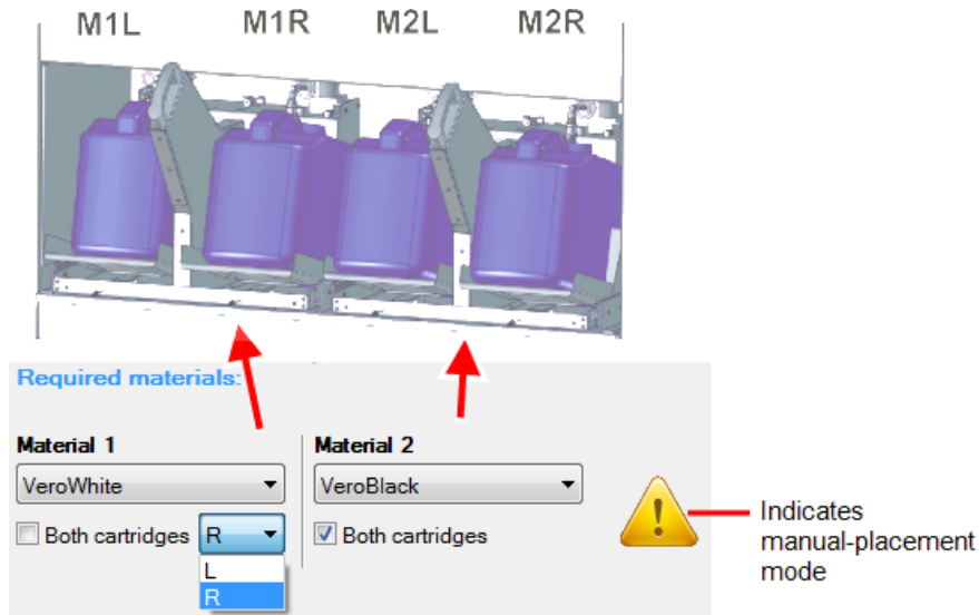
Figure 6-15 Manual cartridge placement
