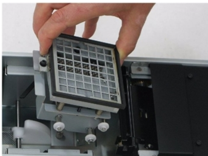
Figure 6-29 Purge unit waste collector
