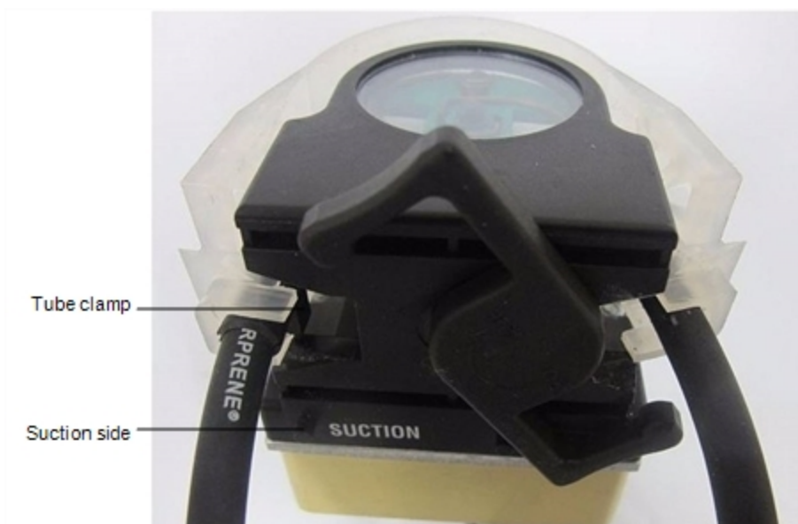
Figure 6-95 Tube clamp on SUCTION side of pump
