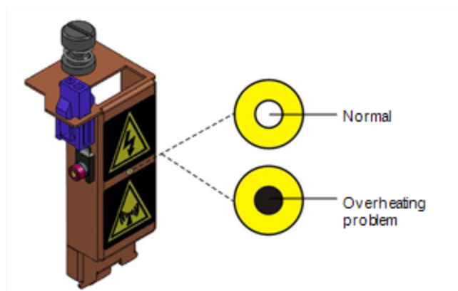
Figure 6-20 Heat-sensitive label on UV lamp cover
