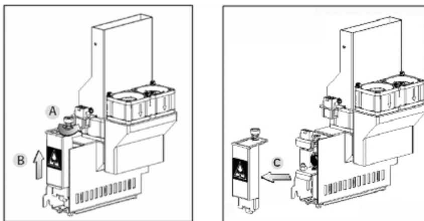
Figure 6-104 Removing the UV lamp cover
