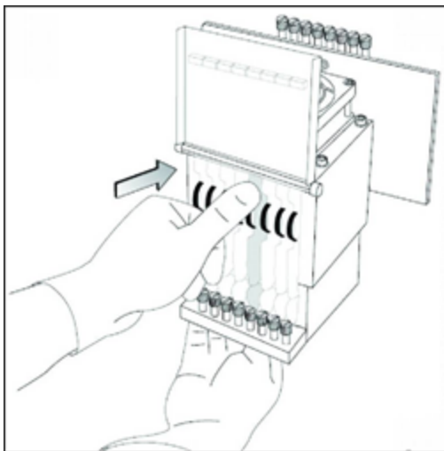
Figure 6-76 Inserting the print-head driver card into its socket
