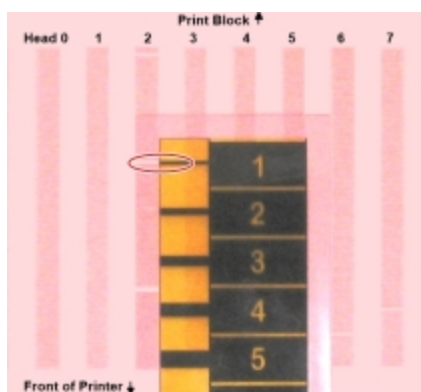
Figure 6-57 Inspecting the Pattern Test
