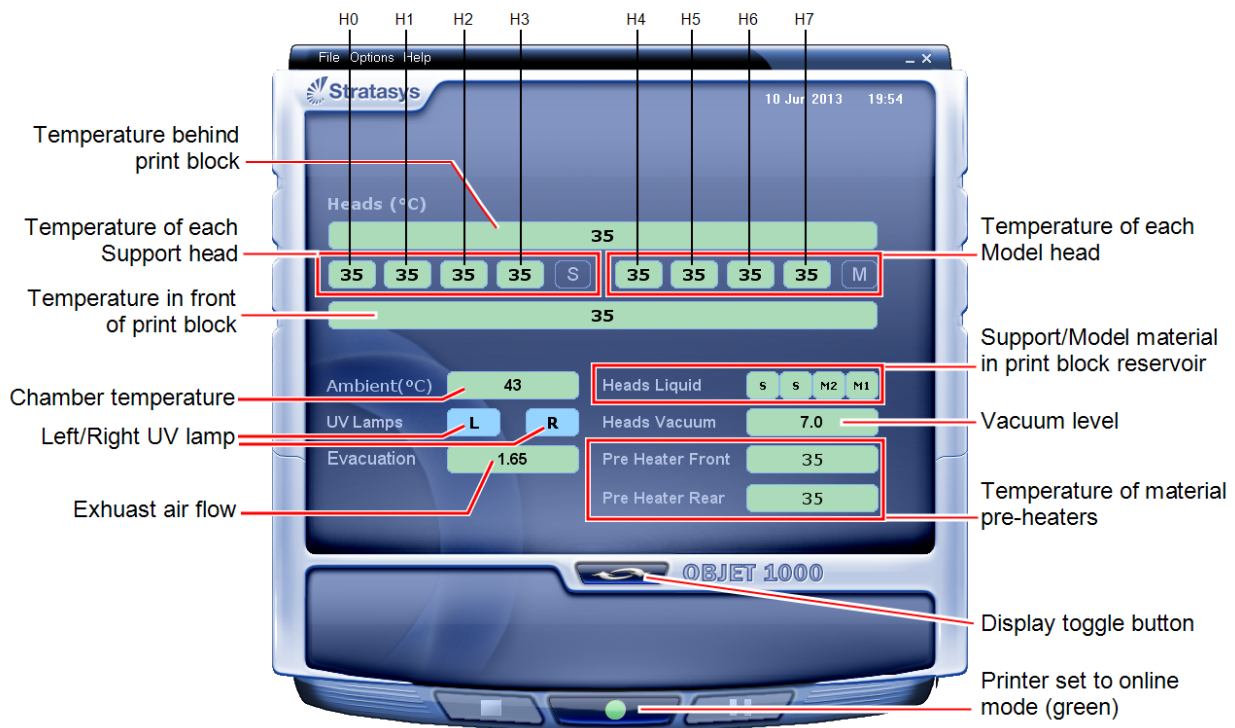
Figure 6-5 Printer status
