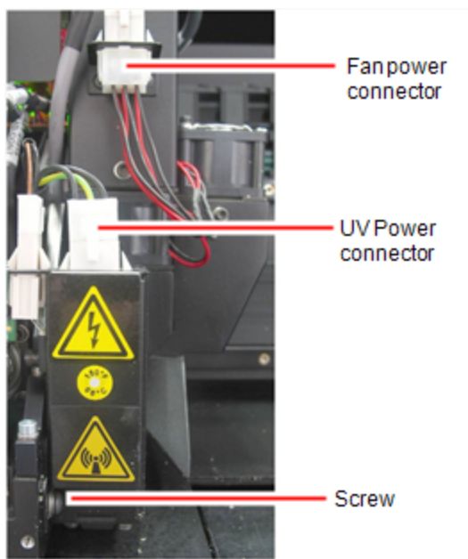
Figure 6-31 Disconnecting the right UV assembly
