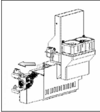
Figure 6-105 Removing the UV lamp reflector
