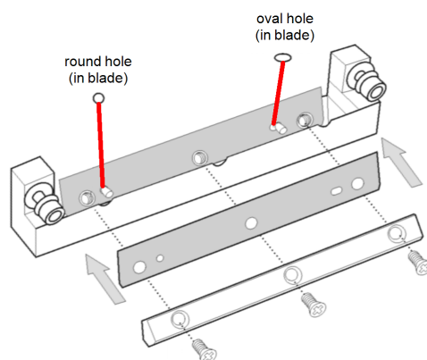
Figure 6-41 Inserting the new roller scraper blade
