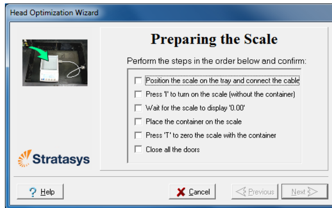
Figure 6-60 Setting up the Head Optimization scale
