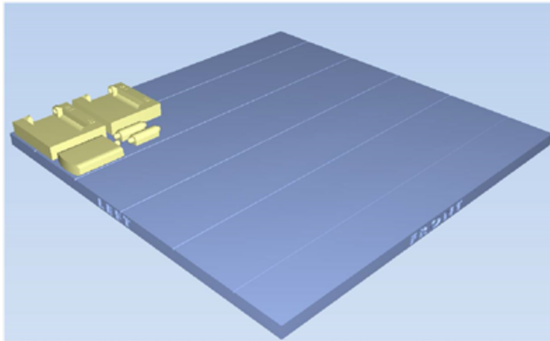
Figure 5-34 Tray arrangement after applying Automatic Placement
