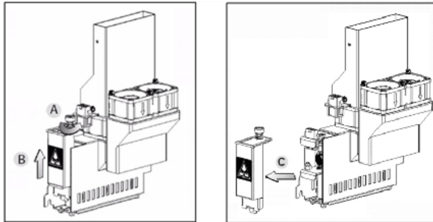
Figure 6-114 Removing the UV lamp cover
