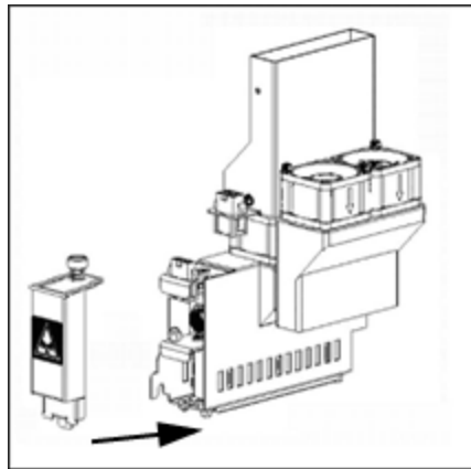
Figure 6-124 Replacing the UV lamp cover
