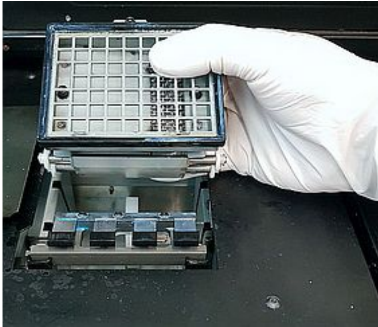
Figure 6-33 Purge unit waste collector
