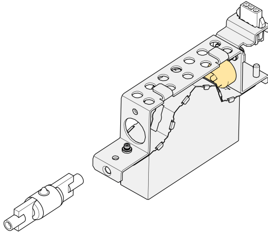
Figure 6-117 Removing the UV lamp bulb
