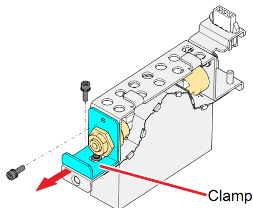
Figure 6-116 Removing the UV lamp clamp
