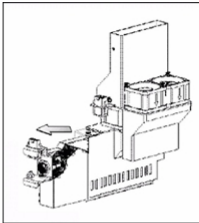
Figure 6-115 Removing the UV lamp reflector
