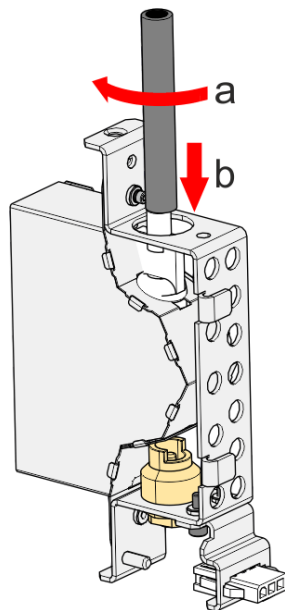
Figure 6-120 Twisting the tube and inserting the UV lamp
