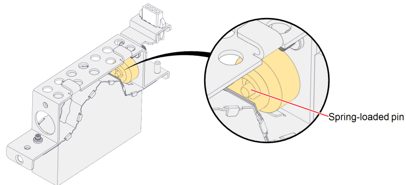
Figure 6-118 Spring-loaded pin
