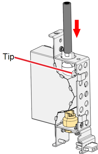
Figure 6-119 Pushing the new UV bulb into the UV reflector
