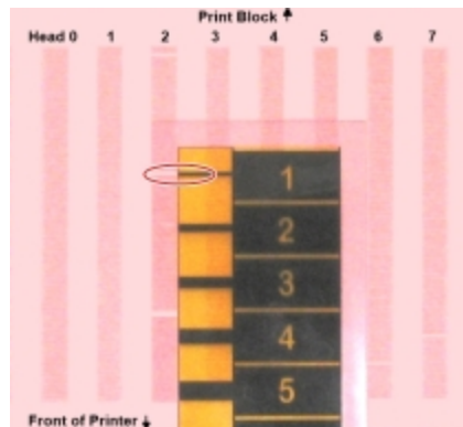
Figure 6-64 Inspecting the Pattern Test
