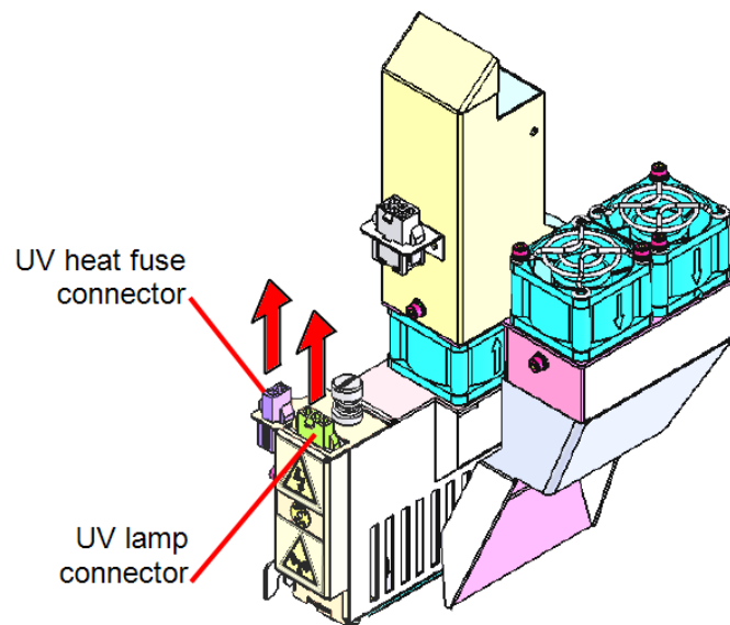
Figure 6-113 Disconnecting the UV lamp
