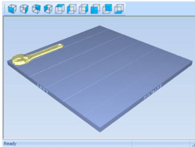
Figure 5-116 Job Preview
