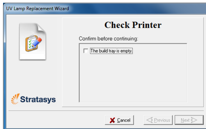
Figure 6-111 Tray confirmation
