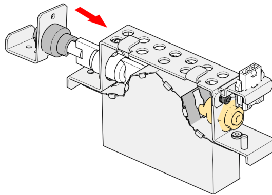
Figure 6-121 Pushing the UV lamp into place
