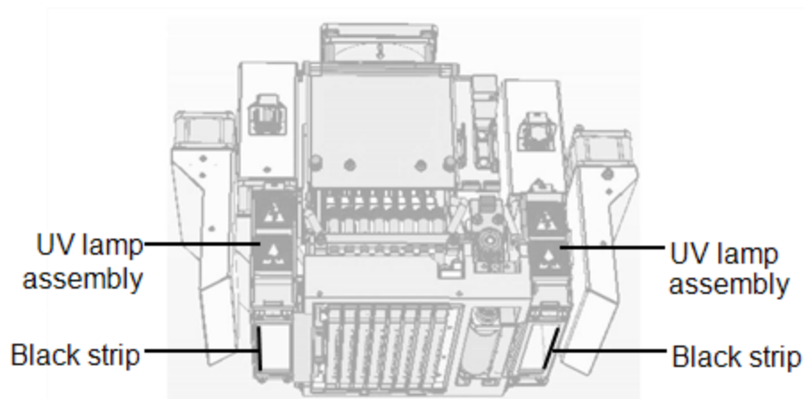
Figure 6-123 Print block and UV lamp assembly, showing correct placement of black strip
