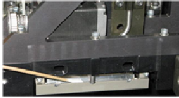
Figure 6-42 Cleaning the roller waste collector
