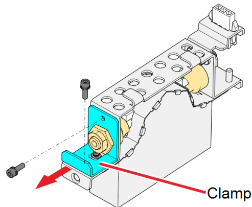
Figure 6-122 Attaching the UV lamp clamp
