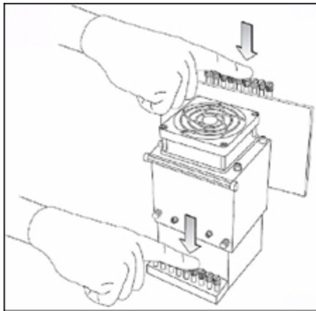
Figure 6-77 Releasing the print head
