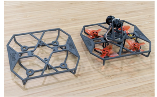
A camera drone frame (left) 3D printed with SAF technology and the completed assembly (right).
